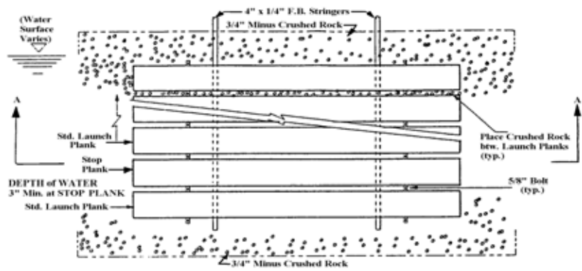
CONCRETE LAUNCH-PLAN VIEW Figure 23 No Scale
